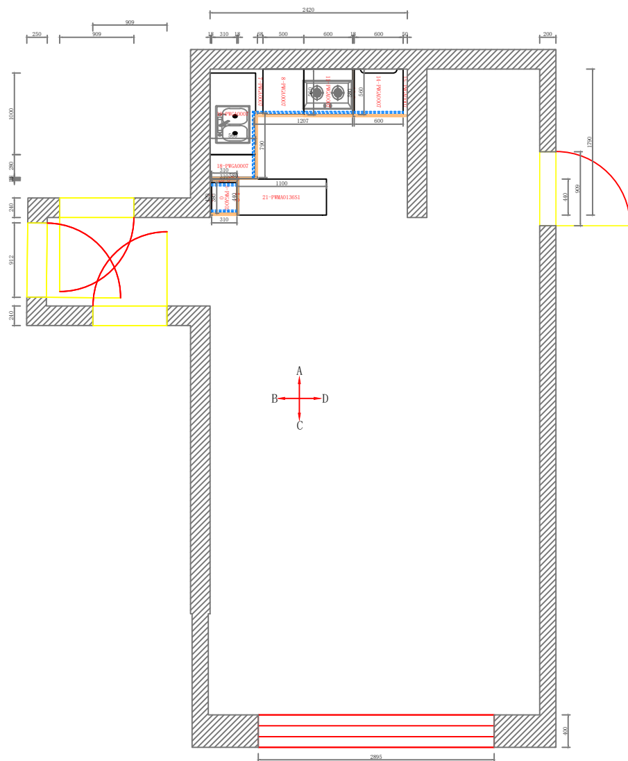
Base cabinet plan
