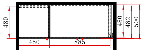
Top view_Lower cabinet
