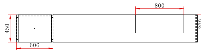
Top view_Lower cabinet
